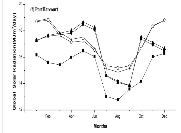
Figures 2 a-f: Comparison between the Observed and the Predicted Monthly Average Global Solar Radiation, \overline{R_s} for (a, b) Kano-Sahelian, (c) Lokoja-Midland, (d, e) Jos-Guinea Savannah, and (f) PortHarcourt-Coastal Region.
