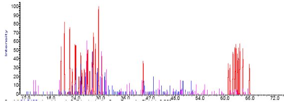
Figure 12: X-ray Diffraction Spectra for PbS Thin Film.
