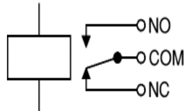
Figure 2: A Relay Switch Representation in the ISBAS.
