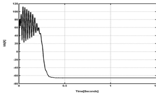
Figure 13: Plot of i_{ds} against Time.
