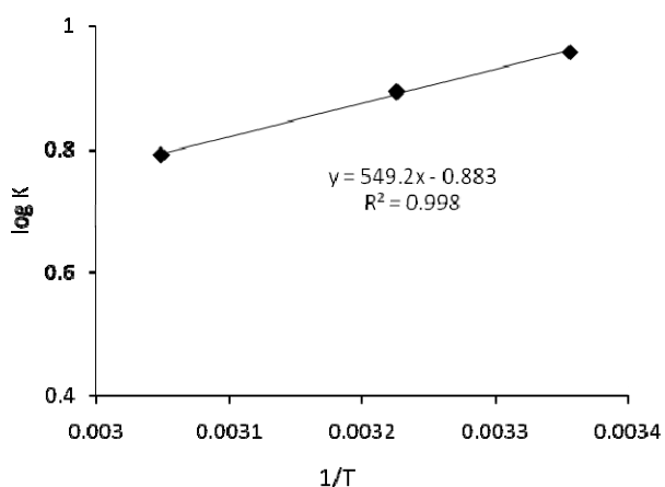
Figure 11: Thermodynamic Profile of Sorption of Pb(II) ions by Talinum triangulare at 30 mg Dose, pH 4, 30 minute Agitation time, and 0.3 mM Initial Metal Ion Concentration.
